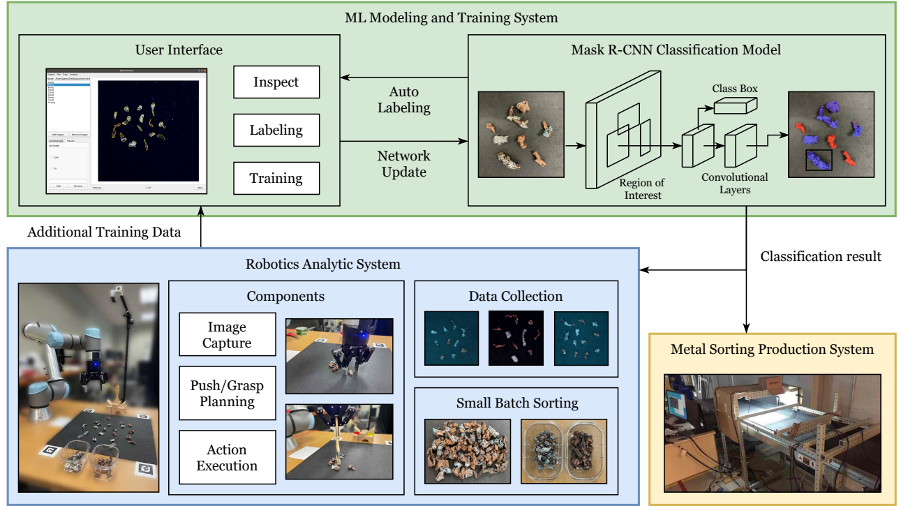
Fig. 3: System architecture. The system has three main components. The ML modeling and training system is composed of a Mask R-CNN [28] classification model, which outputs accurate metal scrap classification result, and a user interface, which is used to inspect and label the training data for Mask R-CNN. To improve the labeling efficiency, the classification model can automatically label the training data for further manual tuning. The second part, named robotics analytic system, employs a camera and a push and grasp policy to handle and analyze small batches of scraps. The robot analytic system can help generate extra training data for the ML model, or directly sort small batch of metal scraps with high accuracy and efficiency. The third part is a conveyor belt production system for large scale metal sorting. Both the robotics and production systems use the Mask R-CNN model to perform object classification.
